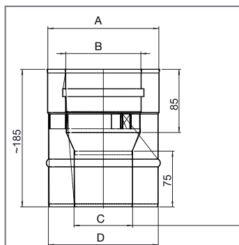
Verloop 79/148 - 100/150 / ATWIN464
